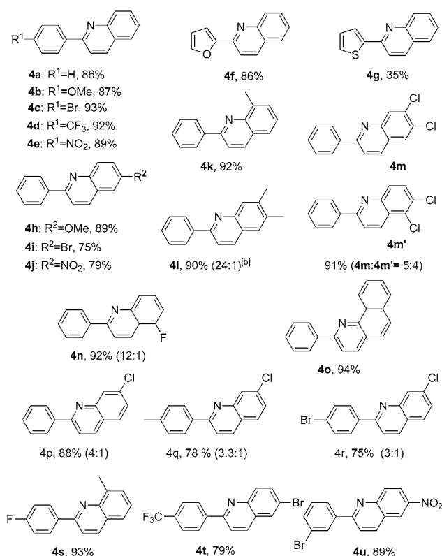
Scheme 2. Synthesis of substituted 2-phenylquinolines. Reaction conditions: aldehyde 1 (0.5 mmol), arylamine 2 (0.5 mmol), acrylic acid 3a (1 mmol), PdCl 2 (0.025 mol, 5 mol%), LiBr·H 2 O (0.5 mmol, 1 equiv), in acetonitrile (2 mL) at 60 °C in air for 8 h. Yields of isolated products are reported.
