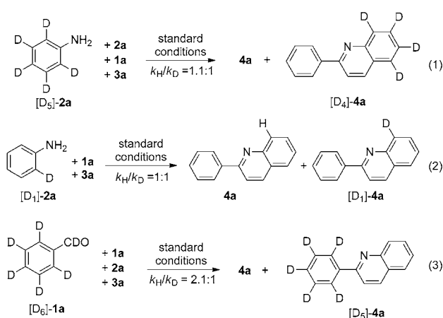
Scheme 4. Kinetic isotope effect (KIE) experiment.
