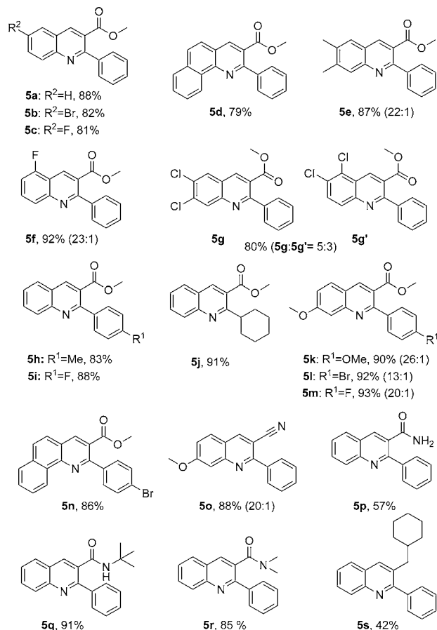
Scheme 3. Synthesis of a variety of substituted quinolines. Reaction conditions: aldehyde 1 (0.5 mmol), arylamine 2 (0.5 mmol), terminal olefin 3 (1 mmol), PdCl 2 (0.025 mol, 5 mol%), LiBr·H 2 O (0.5 mmol, 1 equiv), in acetonitrile (2 mL) at 60 °C in air for 8 h. Yields of isolated products are reported.
